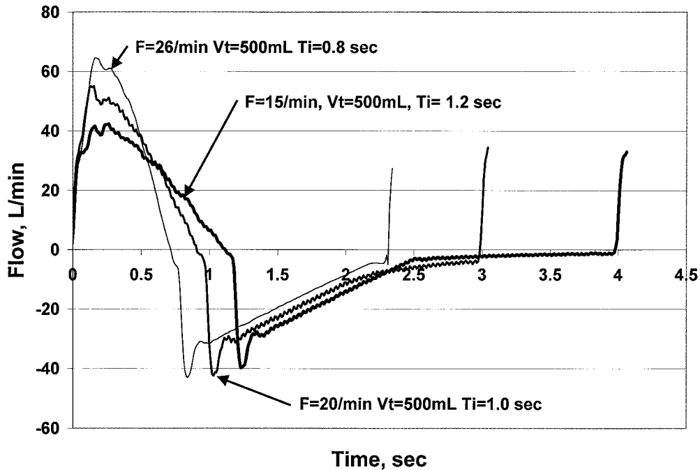
Fig. 2. Flow waveforms for low ( f = 15/\text{min} ), medium ( f = 20/\text{min} ), and high ( f = 26/\text{min} ) respiratory frequency breathing patterns. V_t = tidal volume. T_i = inspiratory time.
